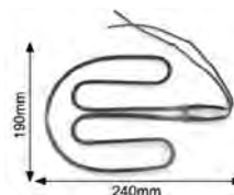
KTE16 ROUND TOASTER ELEMENT 650W 230V Commercial toasters
