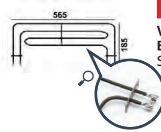
KGE02 OUTER GRILL ELEMENT 2000W Suitable for PRESIDENT
